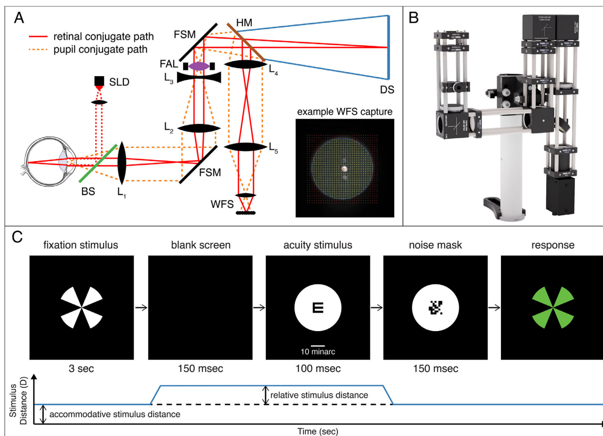
Figure 3. Experimental apparatus and method. (A) Schematic of the apparatus in the main experiment. Infrared light (875 nm) from the superluminescent diode (SLD) is collimated and reflects off a 5:95 R:T beamsplitter (BS) into the eye. The refracted wavefront is imaged via L_1 , front-surface mirror (FSM), and L_2 to be conjugate with the focus-adjustable (FAL) and offset lens L_3 . The IR wavefront is then imaged onto the Shack–Hartmann wavefront sensor (WFS) via a hot mirror (HM), L_4 , and L_5 . The subject views the display screen (DS) through the system and hot mirror. The solid red lines illustrate the retinal-conjugate path and the dashed orange lines the pupil-conjugate path. Inset image is an example WFS capture with spots localized. (B) Rendered model of the display system. The subject’s eye is located to the left and views a display screen to the right (not shown). (C) Experimental procedure for the main experiment with illustrated accommodative stimulus distance, provided by FAL, on bottom. Subjects initially fixate a Maltese cross at the accommodative stimulus distance for that trial. Then the screen is blanked and the optical distance of the screen is changed via the FAL to the desired relative stimulus distance for the acuity stimulus. The change in optical power took \sim 15 ms (as shown by the blue line). An E in one of four orientations is briefly presented. Then the optical distance of the screen is returned to the accommodative stimulus distance while a dynamically changing noise mask is displayed to extinguish an afterimage of the E. A green Maltese cross is then shown, and this signifies that the subject should now indicate the perceived orientation of the E. Once the response is recorded, the white cross reappears and the next trial begins. The white bar in the middle panel indicates 10minarc.
