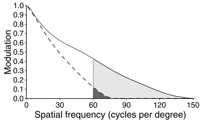
Figure 11. Information beyond the Nyquist limit. Average MTFs for the 3-mm (dashed line) and 5.81-mm (solid line) adaptive-optics-corrected conditions. Vertical dotted line marks the theoretical Nyquist limit of the cone mosaic; shaded areas represents aliasing zone. The aliasing zone is much larger for the 5.81-mm (entire shaded area) than 3-mm condition (darker shaded area).
